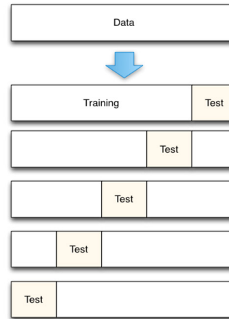
Figure 3. Example of Lasso cross-validation and variable selection. The left figure illustrates how the data set is repeatedly split into a training and test, where a model is built in the "training" set and the performance is checked in the "test" set.
